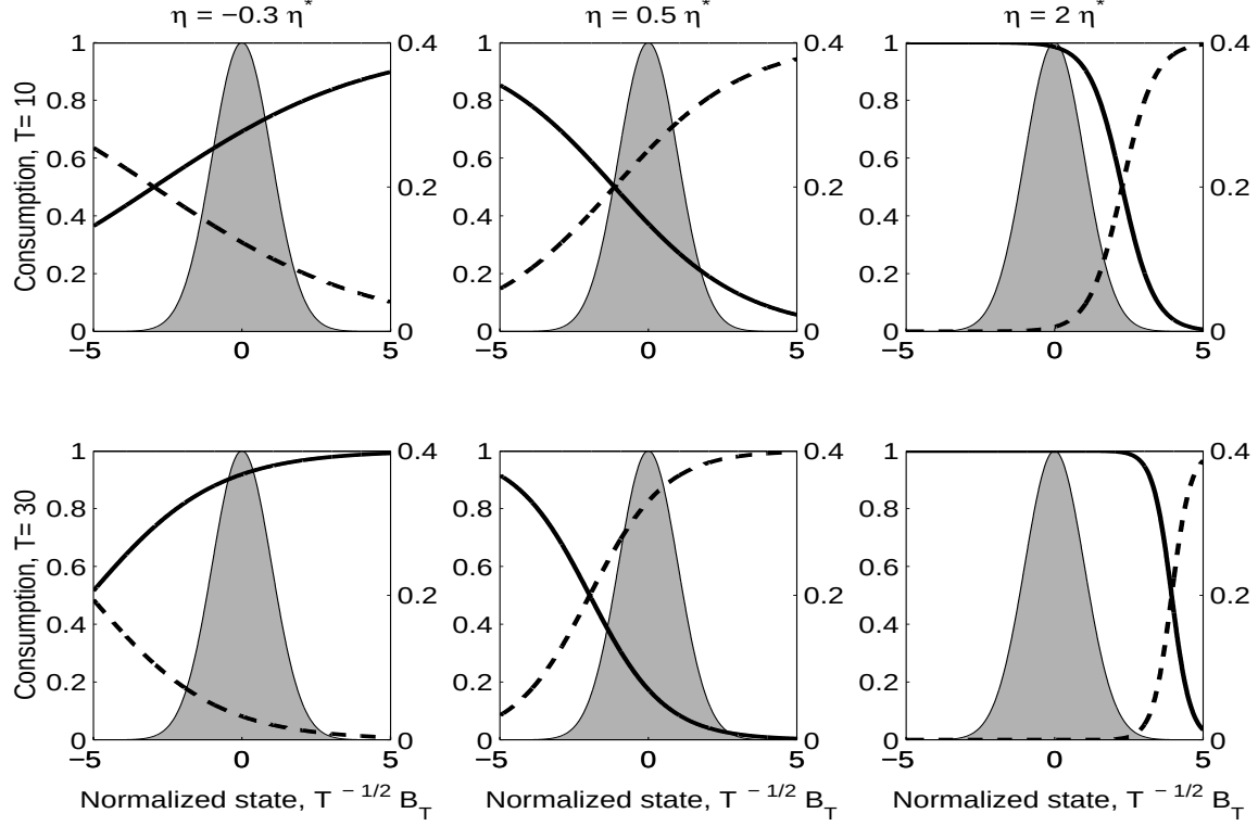
Figure 6: The terminal consumption of rational and irrational traders for different horizon T . We consider two values of T , 10 and 30, respectively. The model parameters are set at \mu = 0.12 , \sigma = 0.18 , and \gamma = 5 . We consider three distinctive cases for the irrational trader's belief: (1) pessimistic, \eta = -0.3\eta^* , (2) moderately optimistic, \eta = 0.5\eta^* , and (3) strongly optimistic, \eta = 2\eta^* . The horizontal axis in all panels is the normalized value of the terminal dividend, i.e., [\ln D_T - (\mu - \frac{1}{2}\sigma^2)T] / (\sigma\sqrt{T}) , which has a standard normal distribution with zero mean and unit variance, shown by the shaded area (vertical axis on the right). The two panels on the left show the terminal consumption, as a fraction of the total consumption, of the rational trader (solid line) and the irrational trader (dashed line) with a pessimistic belief, i.e., C_{r,T}/D_T and C_{n,T}/D_T , for the two values of the horizon, T = 10, 30 , respectively. The two panels in the middle and on the right show the terminal consumption, as a fraction of the total consumption, of the rational trader and the irrational trader with a moderately and strongly optimistic beliefs for the two values of T , respectively.
