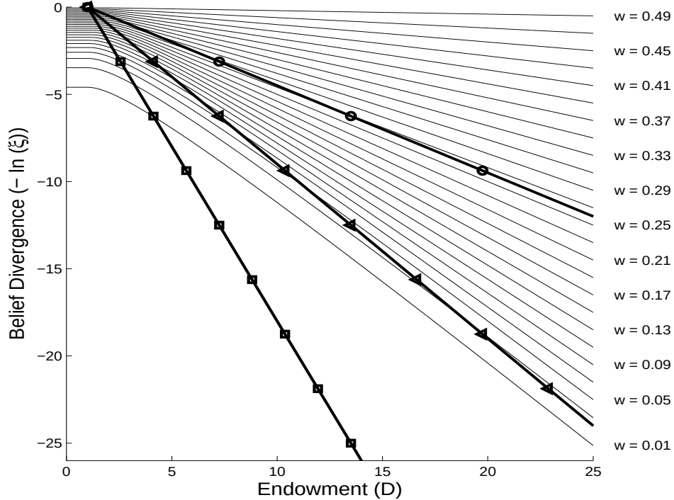
Figure 1: Survival. This figure illustrates survival results in Examples 3.1 and 3.2. We set \lambda = 1 . We plot the aggregate endowment D on the horizontal axis, and the negative of the log of relative belief density, -\ln(\xi) , on the vertical axis. Solid lines are the level curves for the consumption share of agent \mathbb{B} , so that each solid line plots pairs (D, \ln(\xi)) that give rise to a given consumption share w . These pairs can be found by fixing w and plotting the value of \ln(\xi) as a function of D , with the function given by the Pareto optimality condition (8). Labels for agent \mathbb{B} 's consumption share are shown along the right margin. The marked lines show the median path ( Z_t = 0 ) of (D_t, \ln(\xi_t)) for each case in Example 3.1. We choose \delta = 0.5 and set \mu in cases (i), (ii), and (iii) to \delta^2 , \delta^2/4 , and \delta^2/2 respectively. We mark the corresponding median paths with circles, squares, and triangles.
