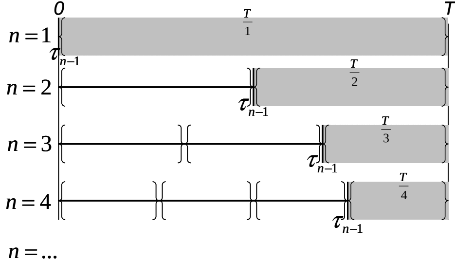
Figure 1: This figure illustrates the construction of the limit in section 3.2. The curly brackets indicate the expected arrival time of Poisson increments, given by \frac{T}{n} = \frac{1}{\lambda(n)} , for different values of n . By construction the expected time of termination E(\tau_n) is equal to T for all n = 1, 2, \dots, \infty . The shaded areas indicate the last “period” before termination. In the paper we study the portfolio choice of the manager in this last period.
